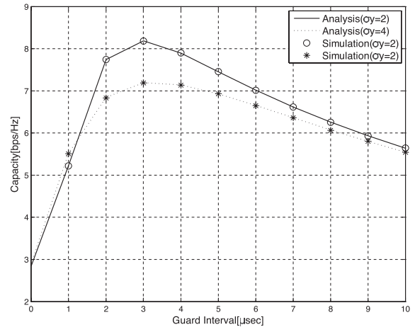
Fig. 2 Capacity for two different standard deviations of log-normal distribution ( \sigma_y ).
